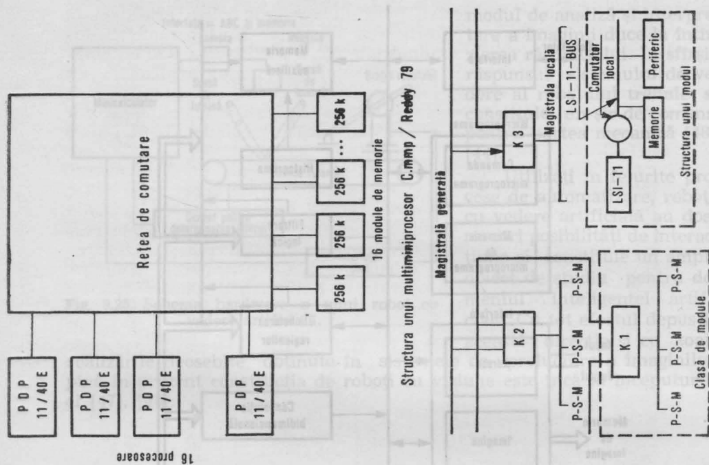
Fig. 9.29. Structura unui sistem multiminicalculator.
